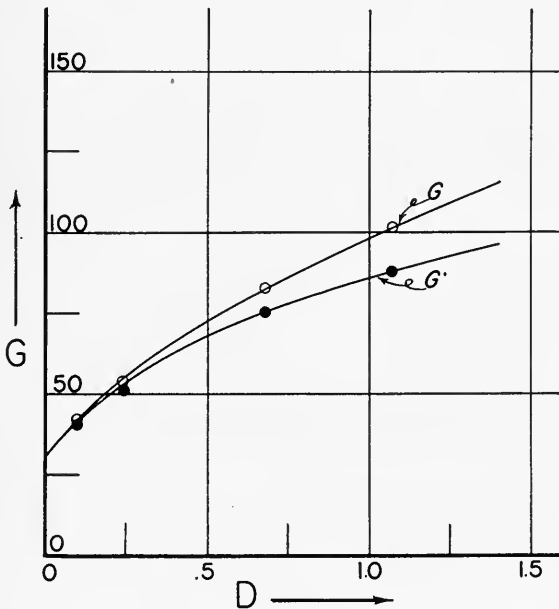
FIG. 11. G - D diagram: The two curves demonstrate the deviations in G observed on a scattering emulsion for higher densities.
